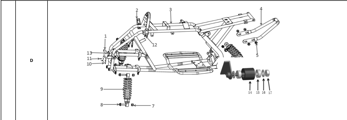
(D车架) FRAME ASSY.
