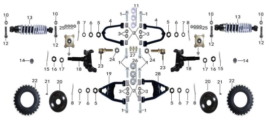
Front suspension system
