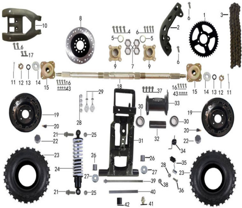
Rear suspension system
